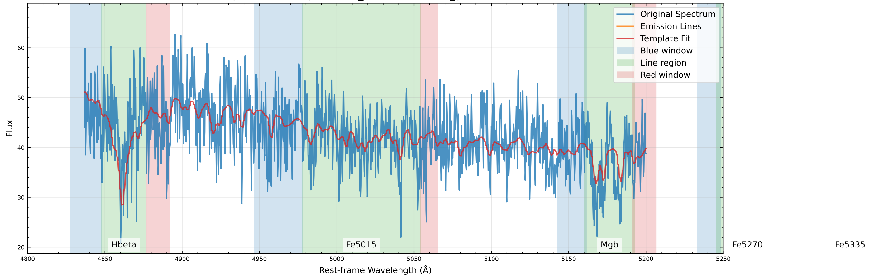
Original Data Comparison (v_star=-7.7 km/s, v_gas=57.7 km/s)
