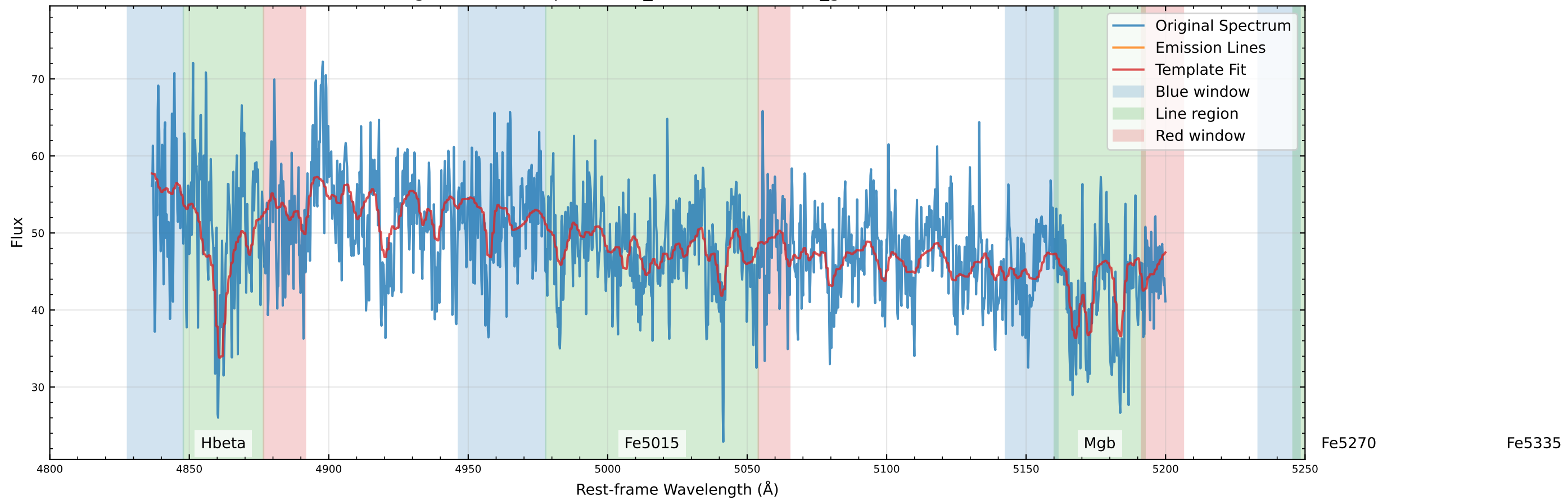
Original Data Comparison (v_star=-12.8 km/s, v_gas=-4.7 km/s)
