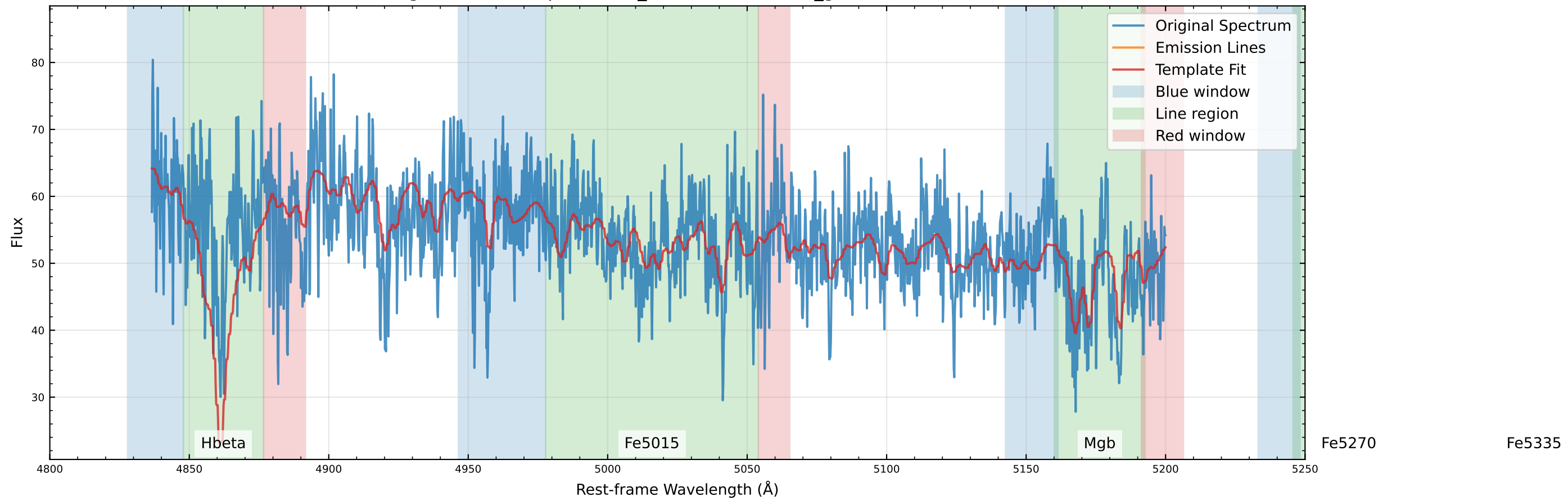
Original Data Comparison (v_star=-19.8 km/s, v_gas=-70.1 km/s)
