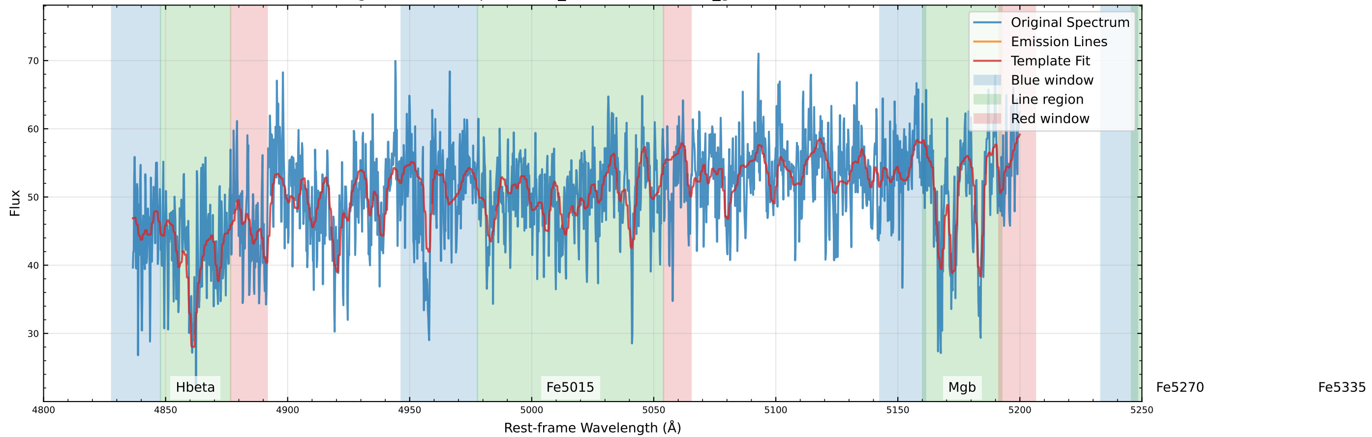
Original Data Comparison (v_star=-16.1 km/s, v_gas=-75.0 km/s)
