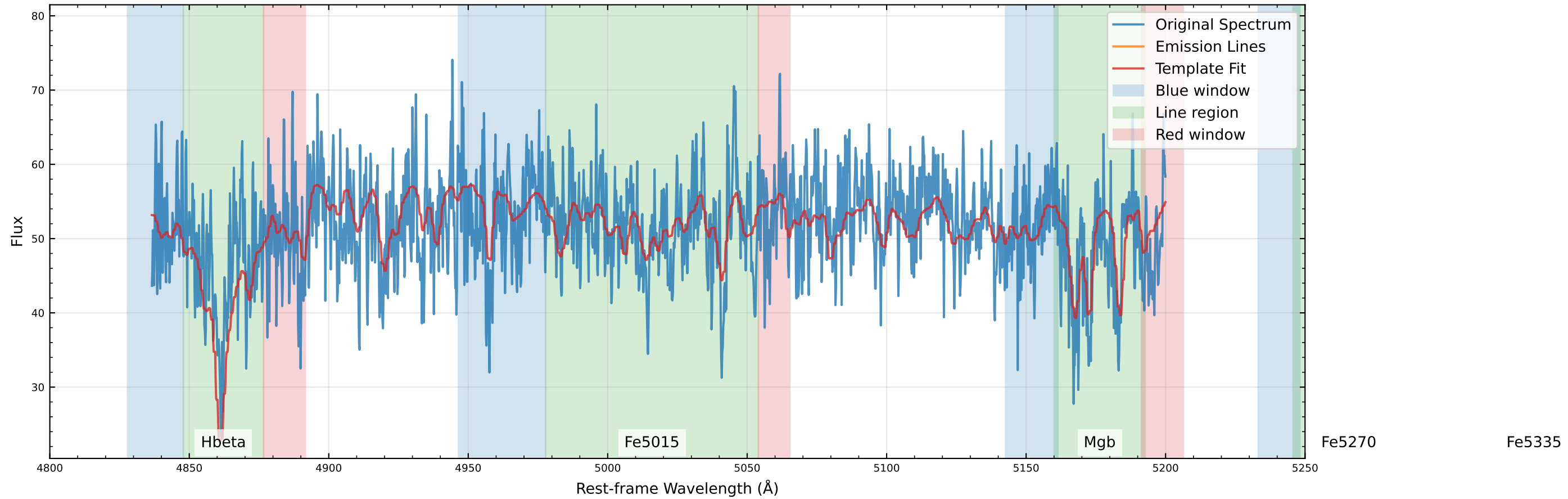
Original Data Comparison (v_star=-17.3 km/s, v_gas=-16.0 km/s)
