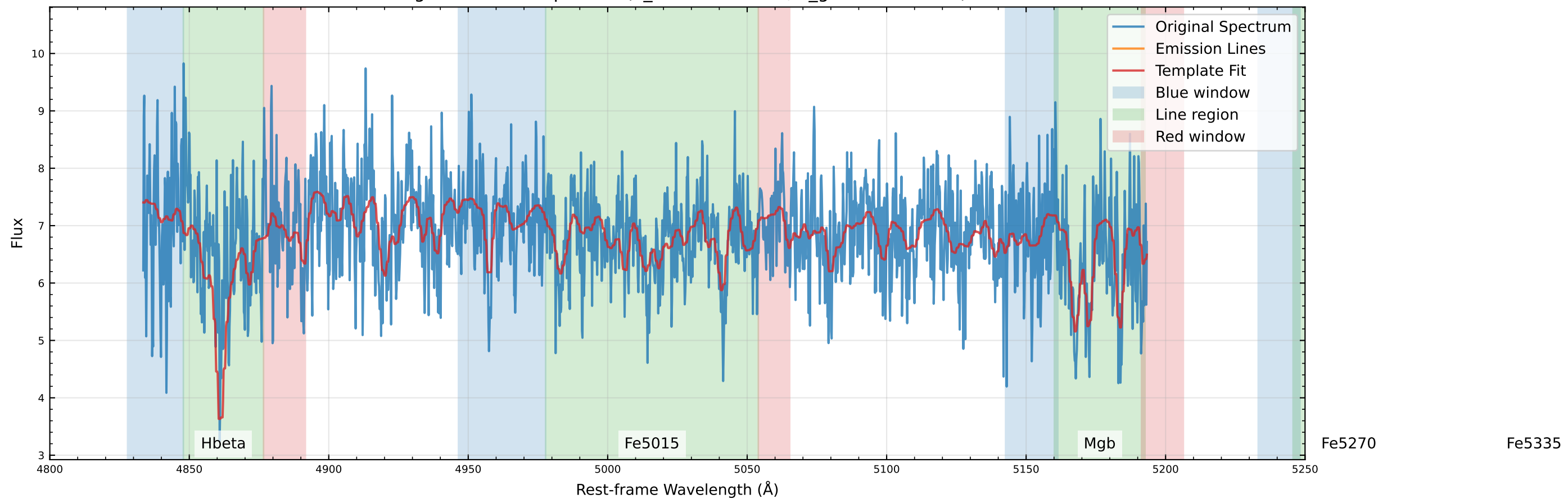
Original Data Comparison (v_star=-0.3 km/s, v_gas=-28.3 km/s)
