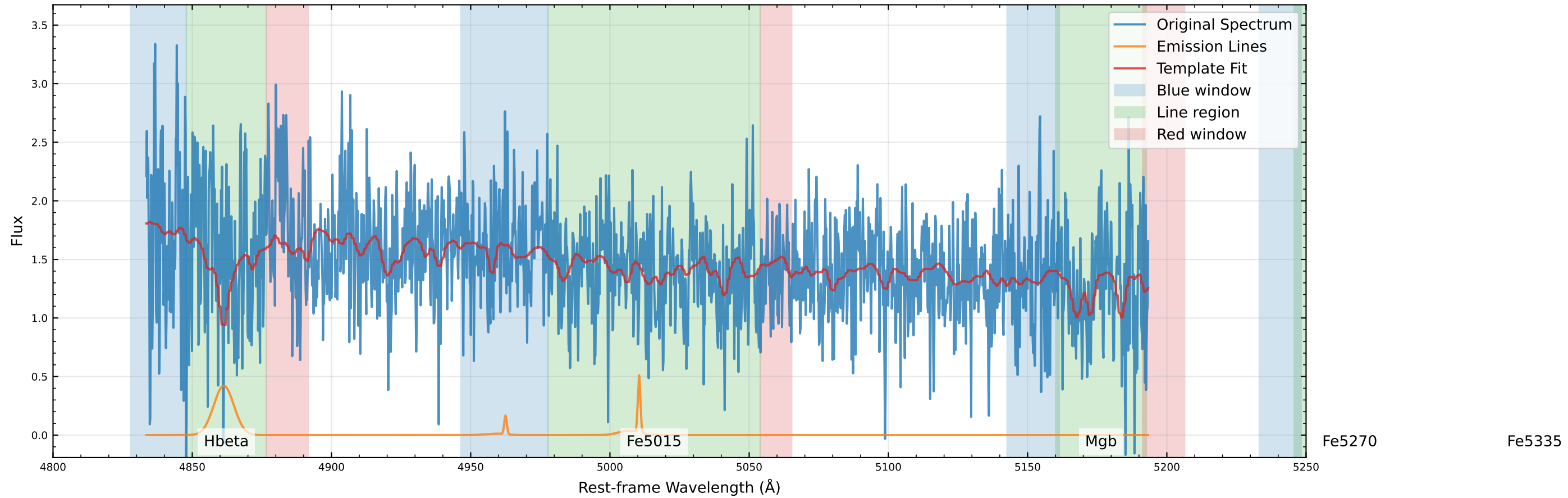
Original Data Comparison (v_star=1.9 km/s, v_gas=-218.2 km/s)
