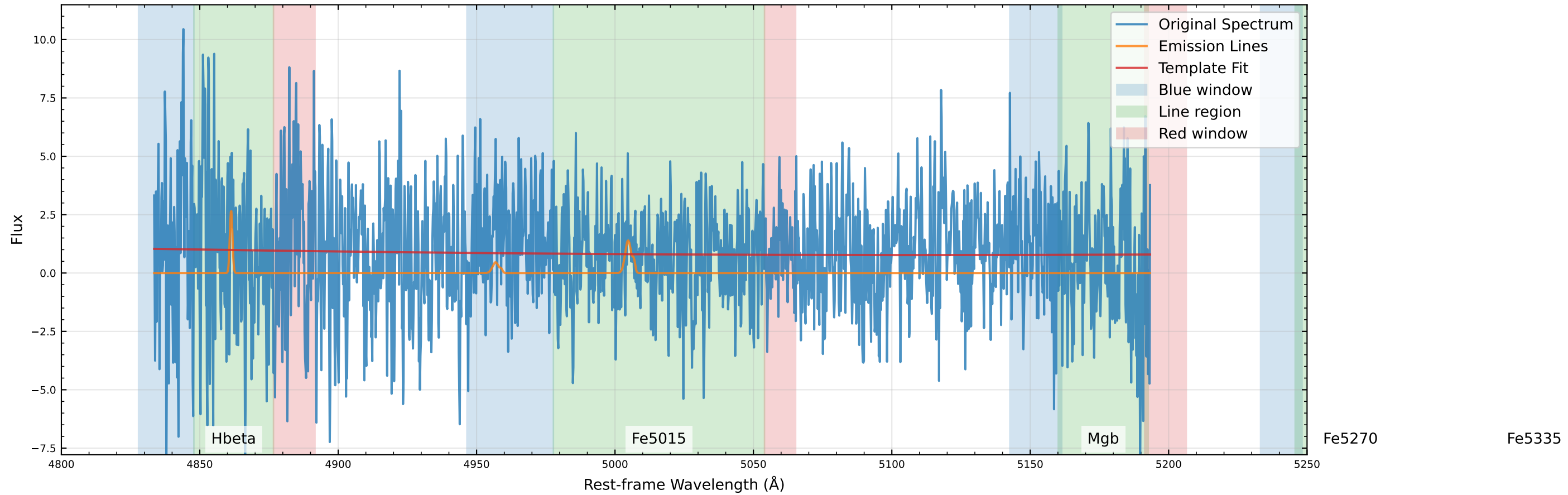
Original Data Comparison (v_star=0.0 km/s, v_gas=15.2 km/s)
