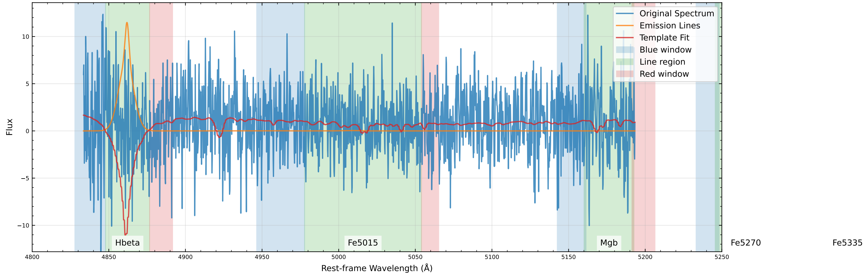
Original Data Comparison (v_star=252.8 km/s, v_gas=230.6 km/s)
