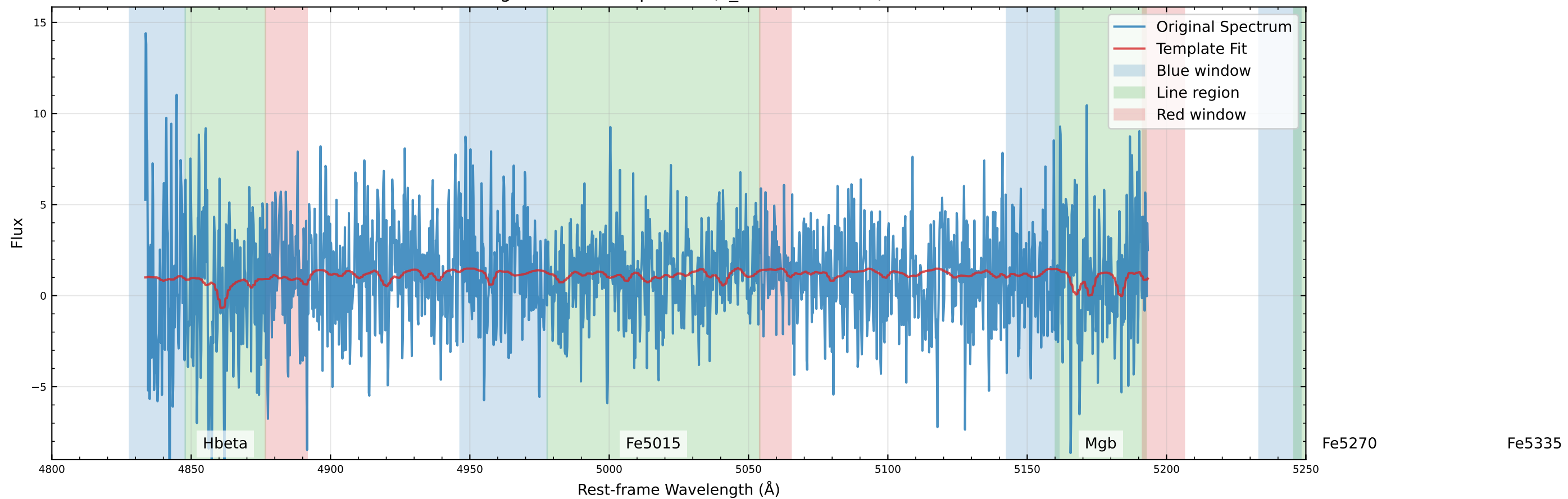
Original Data Comparison (v_star=35.2 km/s)
