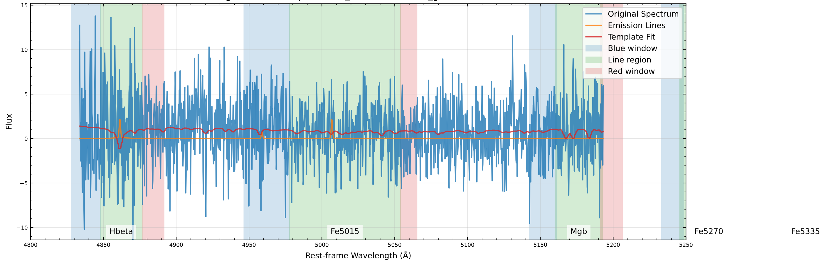
Original Data Comparison (v_star=0.1 km/s, v_gas=-7.8 km/s)
