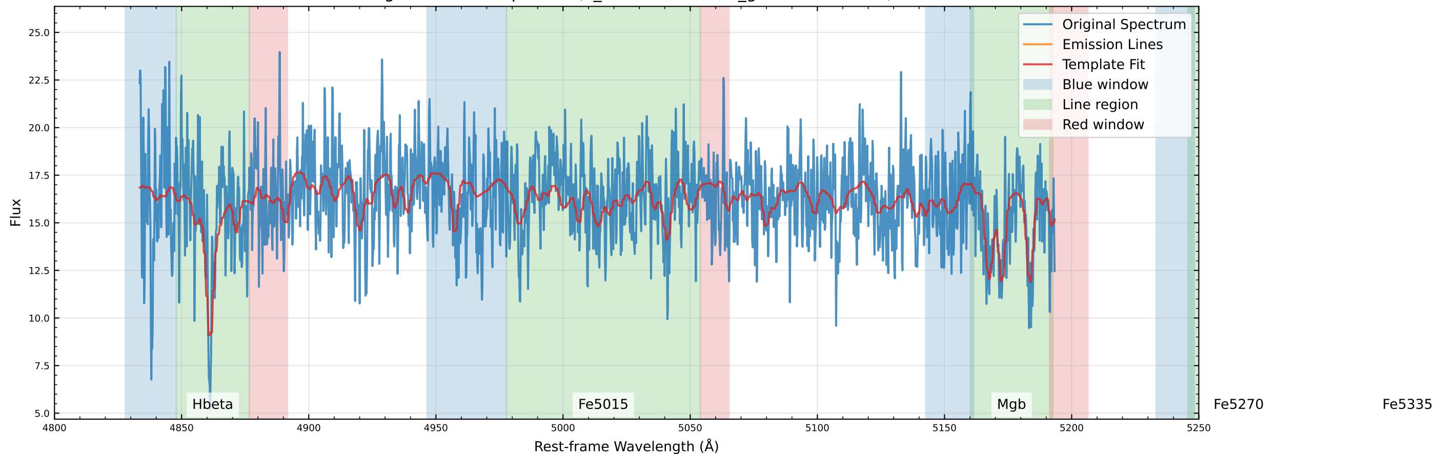
Original Data Comparison (v_star=3.5 km/s, v_gas=-296.5 km/s)
