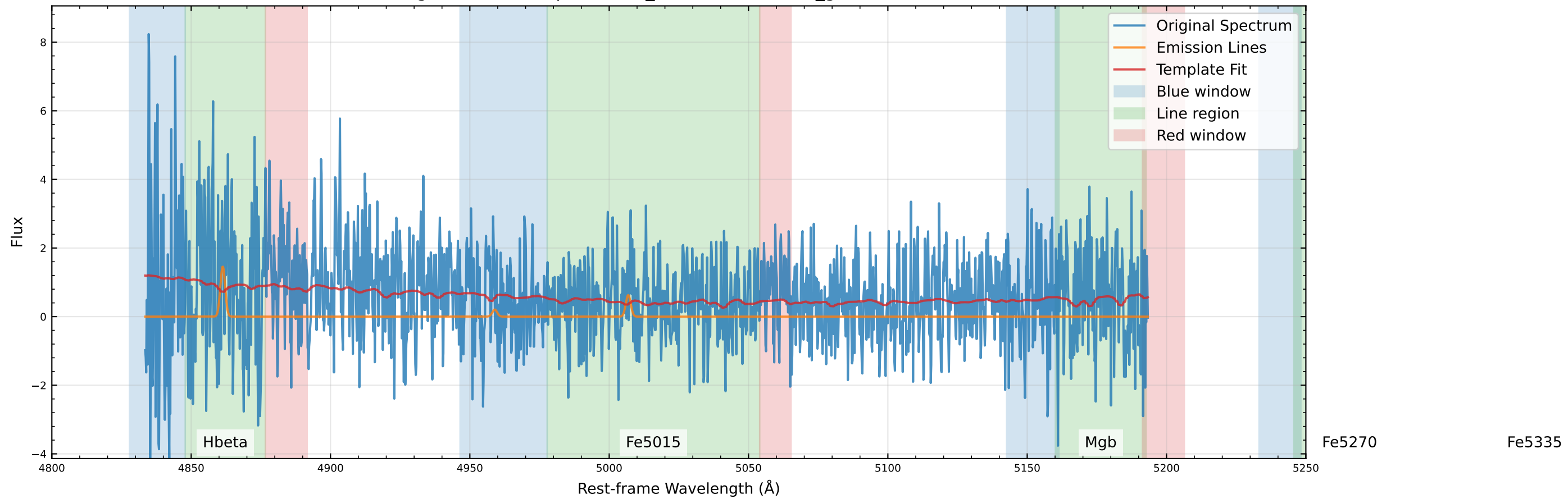
Original Data Comparison (v_star=33.2 km/s, v_gas=49.0 km/s)
