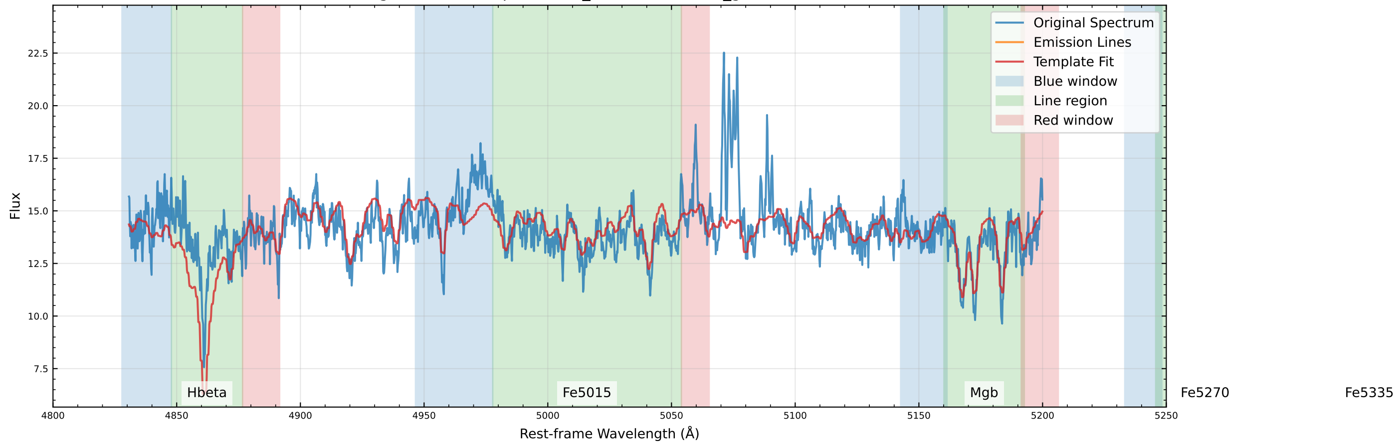
Original Data Comparison (v_star=0.4 km/s, v_gas=-95.7 km/s)
