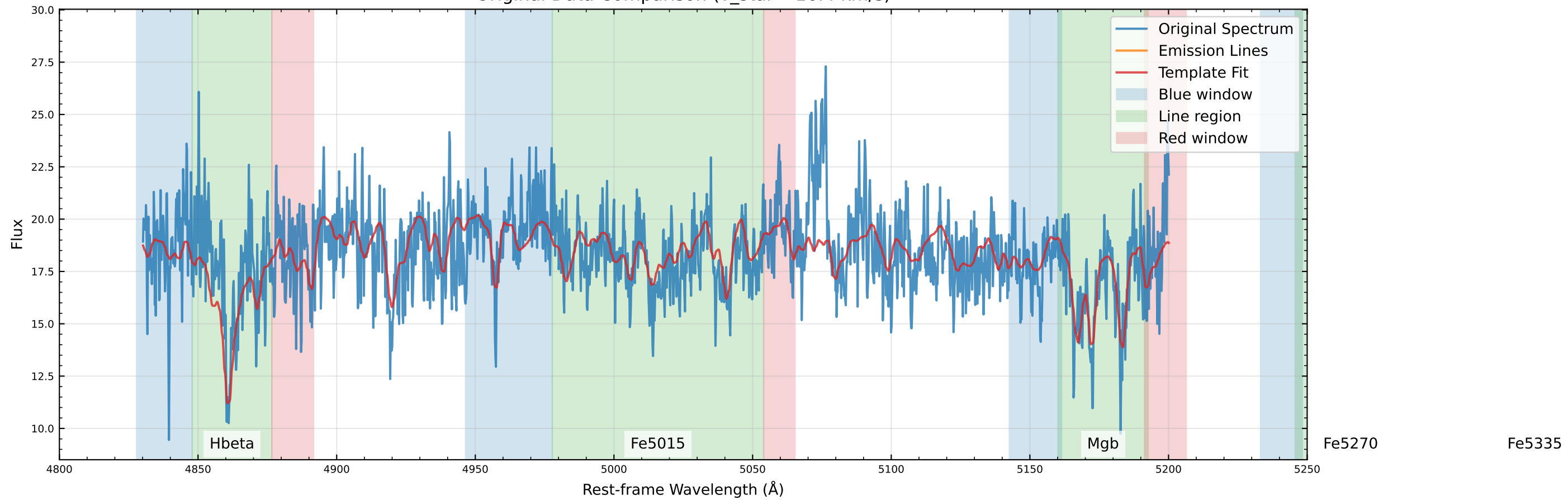
Original Data Comparison (v_star=-16.4 km/s)
