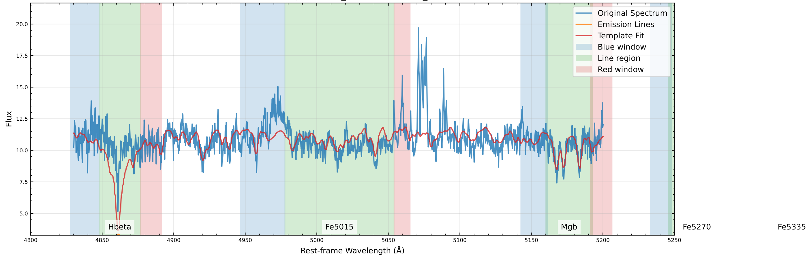
Original Data Comparison (v_star=2.6 km/s, v_gas=6.1 km/s)
