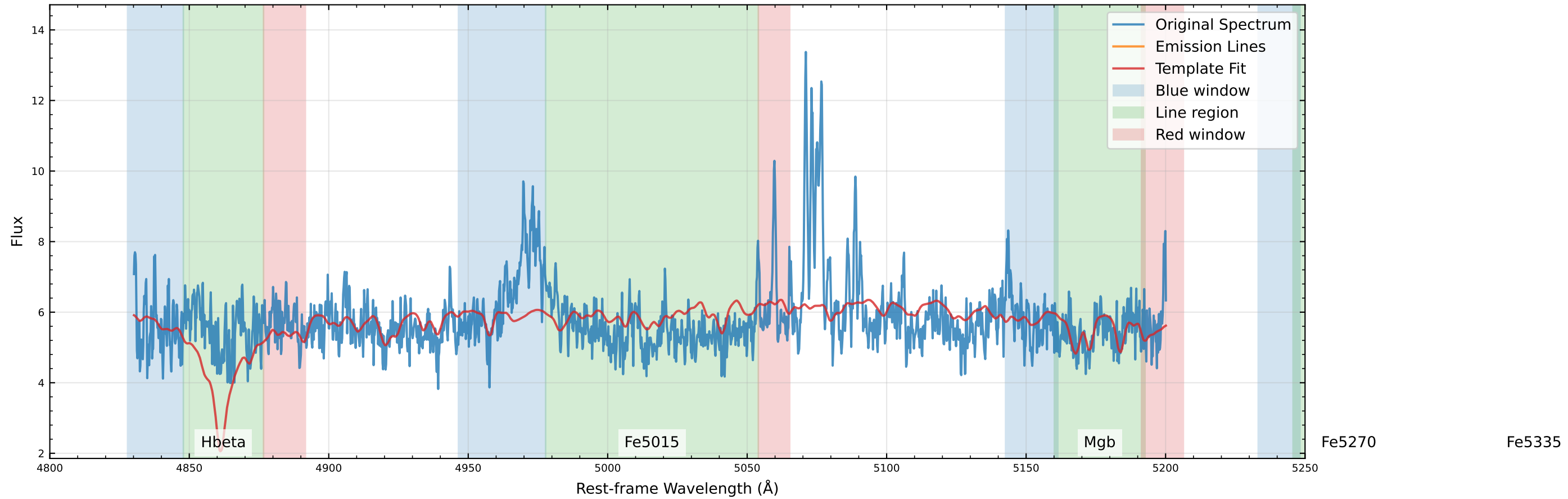
Original Data Comparison (v_star=5.9 km/s, v_gas=-154.7 km/s)
