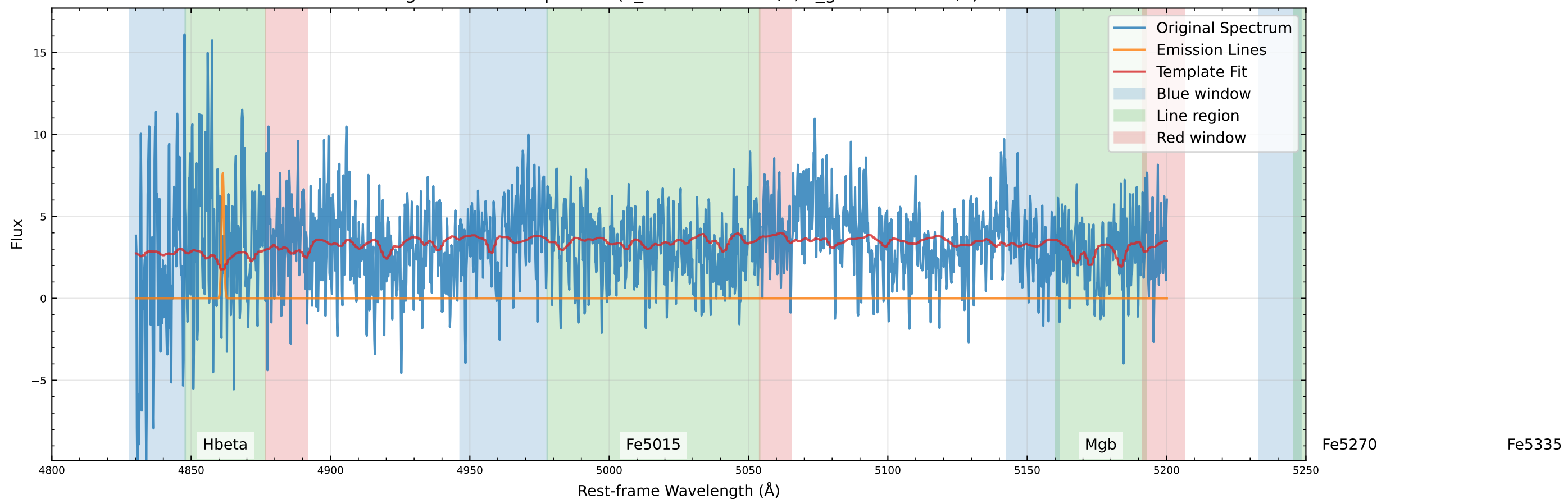
Original Data Comparison (v_star=237.4 km/s, v_gas=438.8 km/s)
