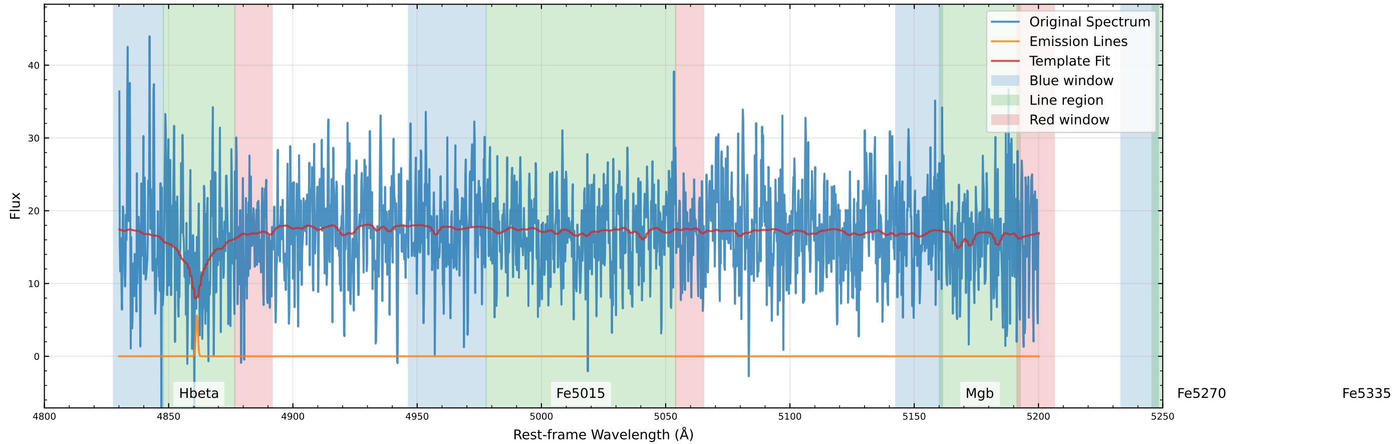
Original Data Comparison (v_star=-22.8 km/s, v_gas=22.4 km/s)
