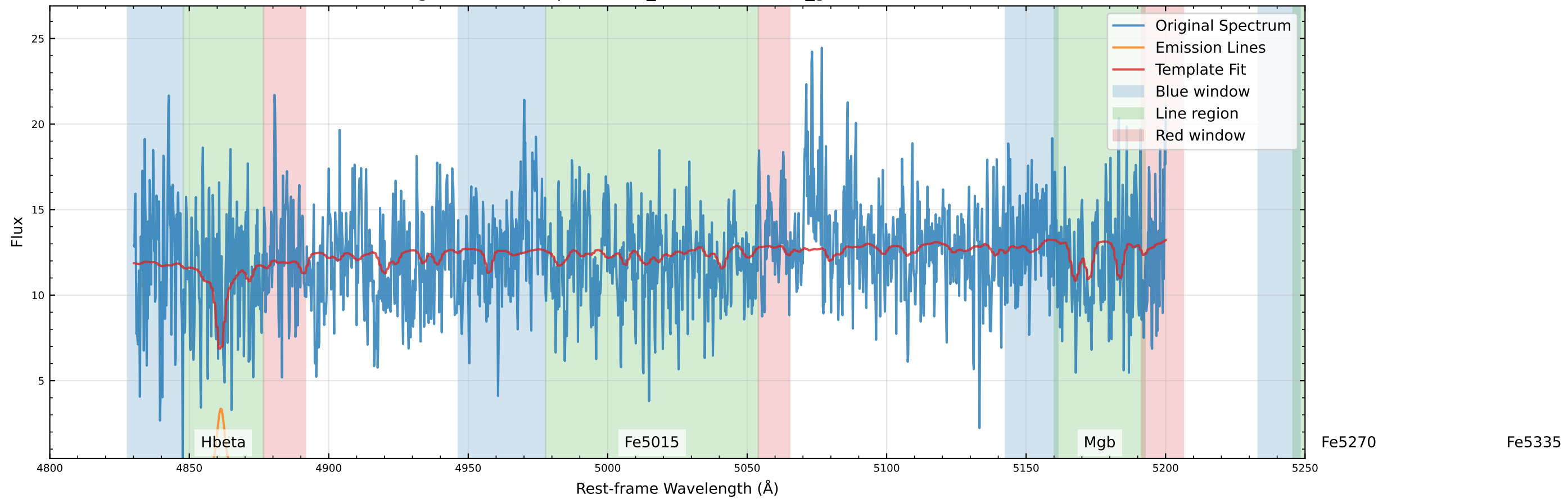
Original Data Comparison (v_star=2.4 km/s, v_gas=-68.8 km/s)
