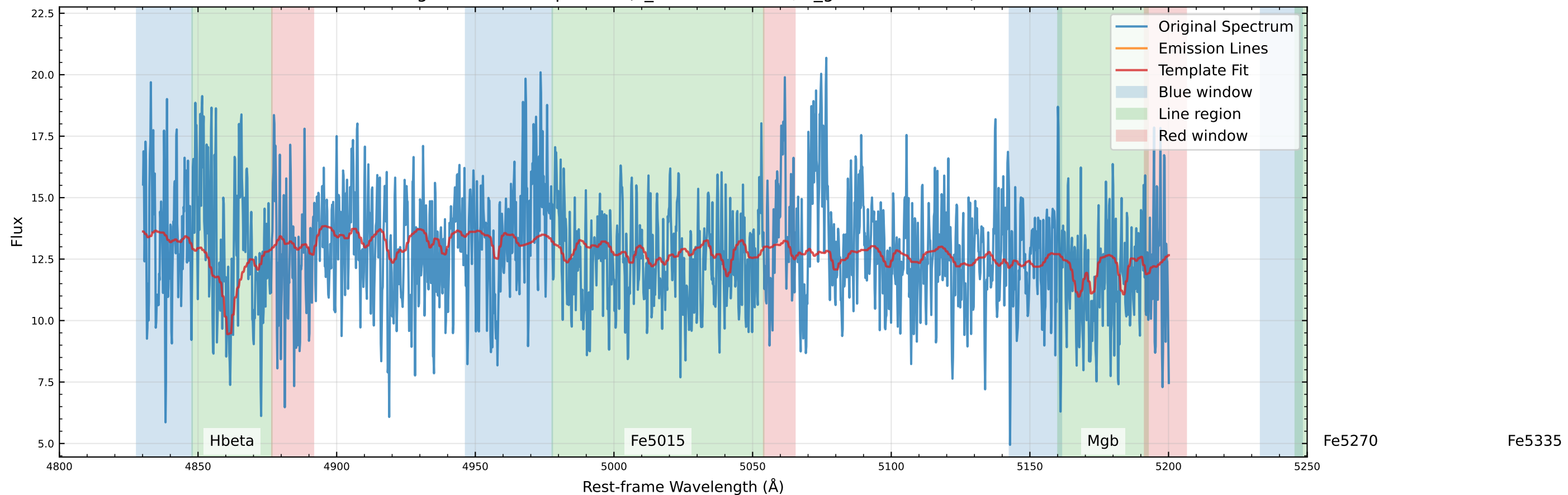
Original Data Comparison (v_star=71.6 km/s, v_gas=227.5 km/s)
