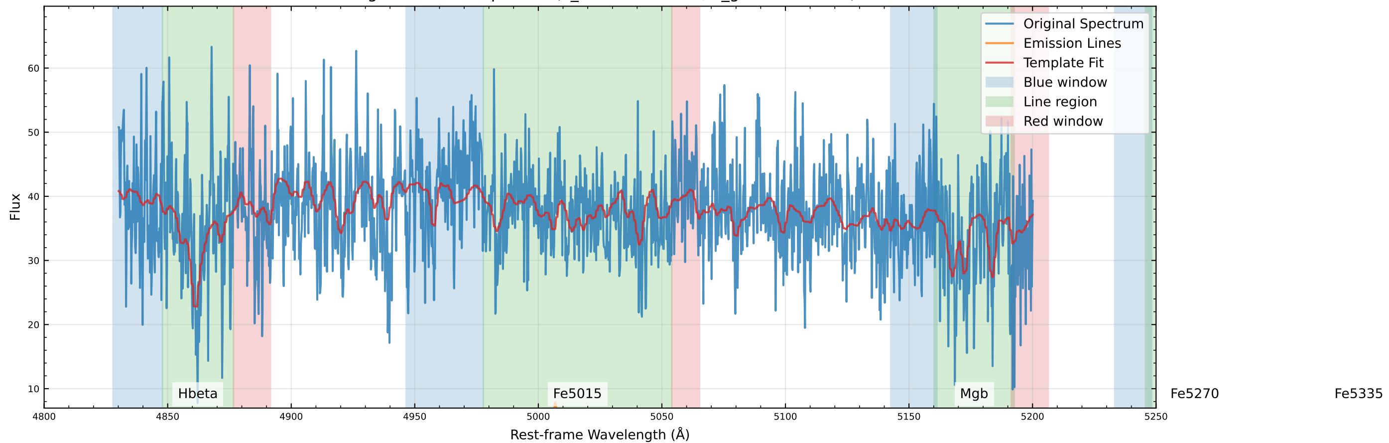
Original Data Comparison (v_star=18.9 km/s, v_gas=55.3 km/s)
