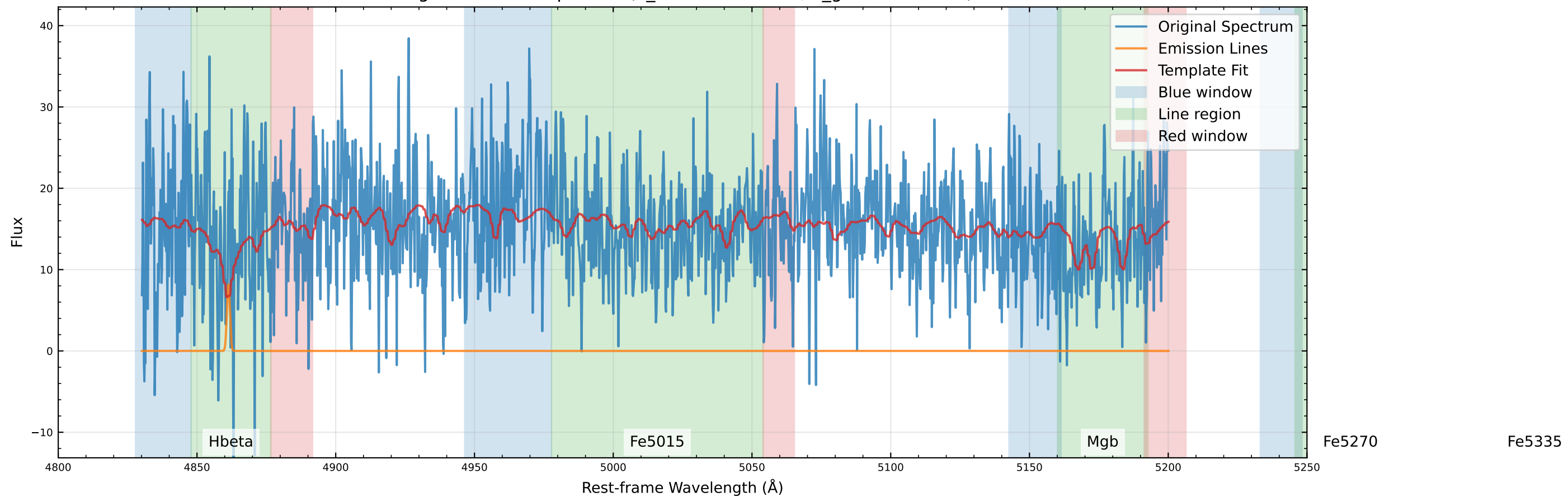
Original Data Comparison (v_star=-46.0 km/s, v_gas=25.1 km/s)
