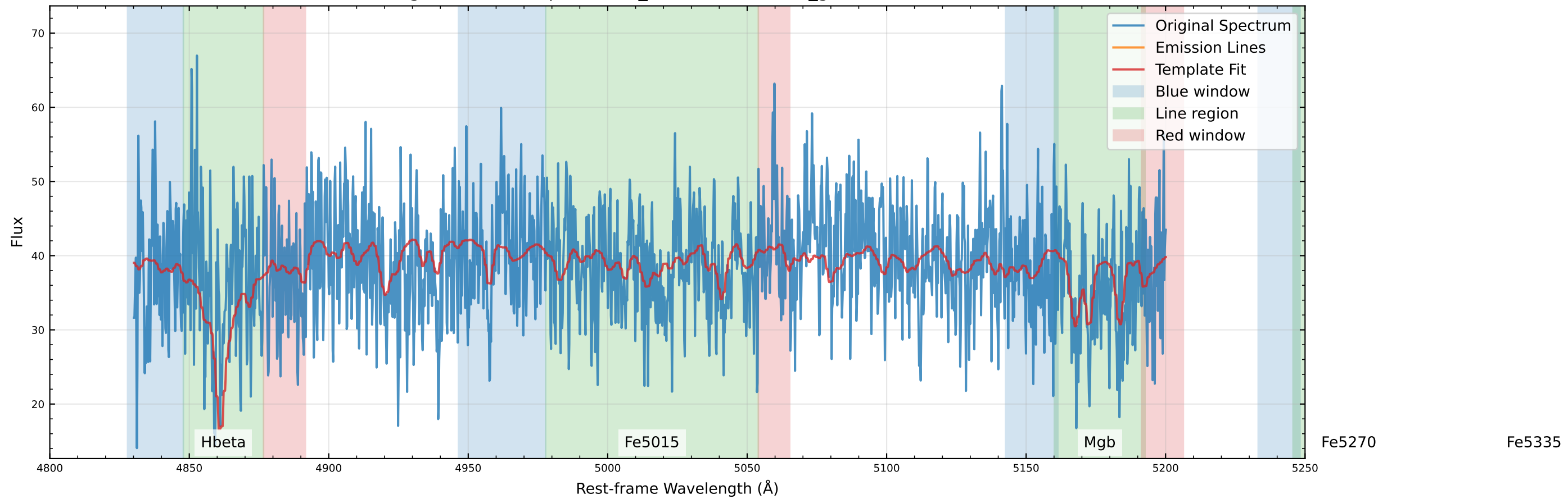
Original Data Comparison ( v_{\text{star}}=25.7 km/s, v_{\text{gas}}=130.9 km/s)
