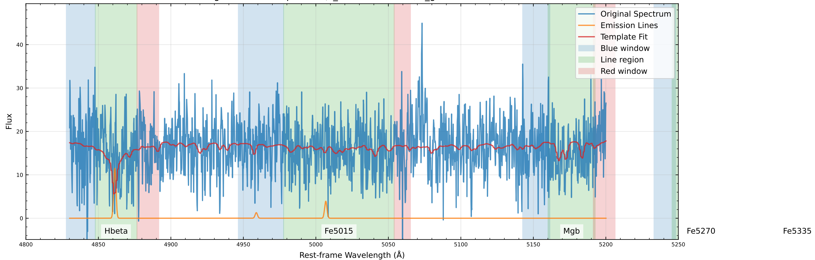
Original Data Comparison (v_star=-15.5 km/s, v_gas=15.6 km/s)
