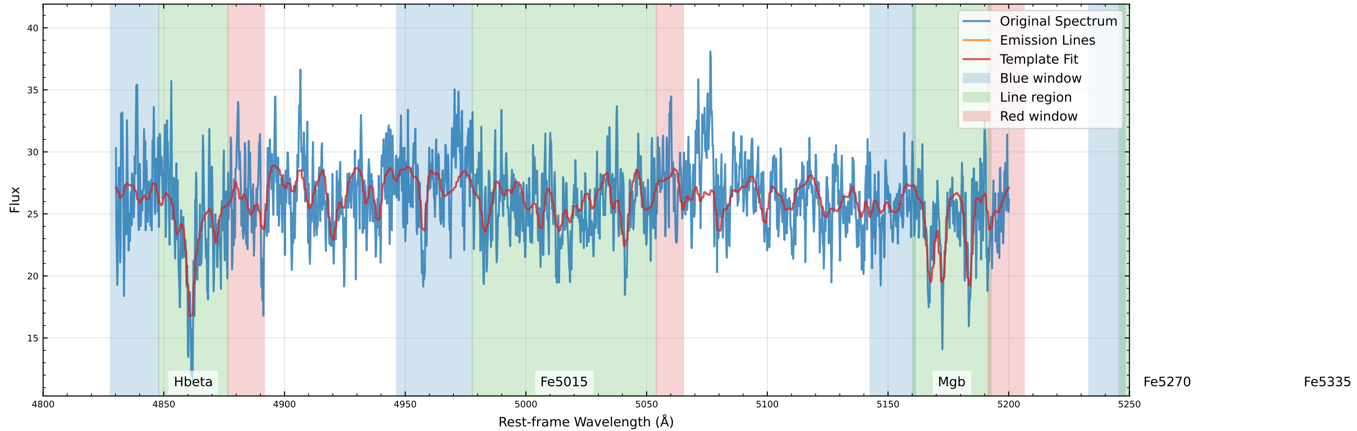
Original Data Comparison (v_star=2.0 km/s, v_gas=62.6 km/s)
