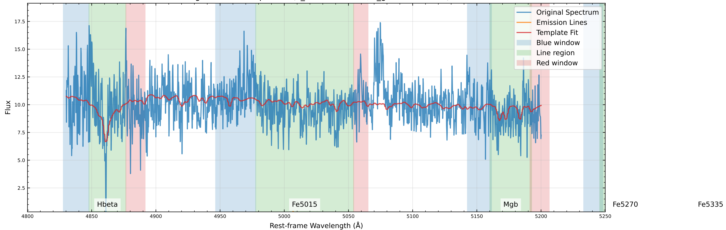
Original Data Comparison (v_star=-3.0 km/s, v_gas=-19.9 km/s)
