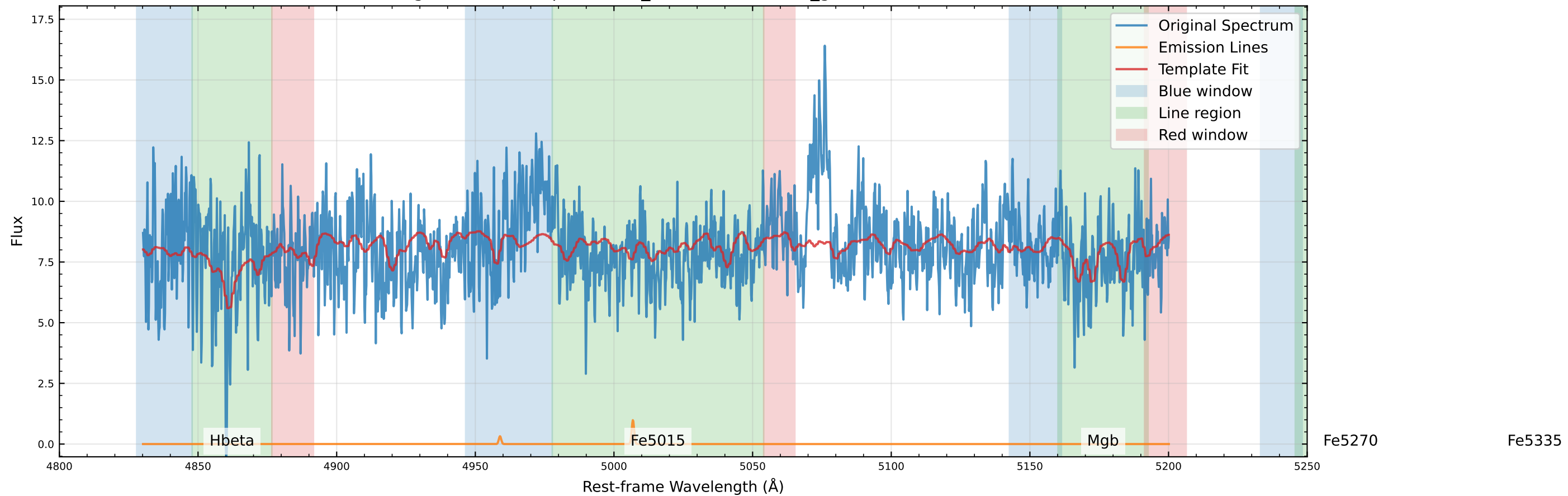
Original Data Comparison (v_star=15.2 km/s, v_gas=-108.7 km/s)
