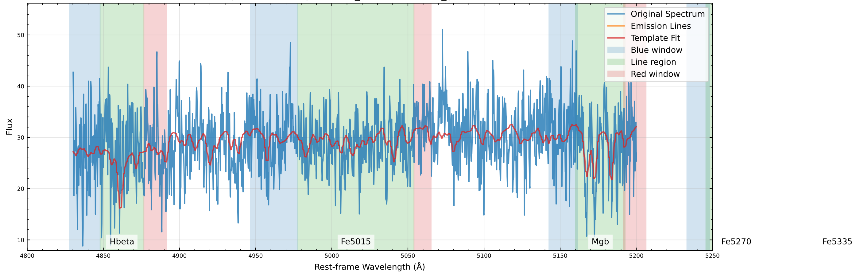
Original Data Comparison (v_star=6.4 km/s, v_gas=21.7 km/s)
