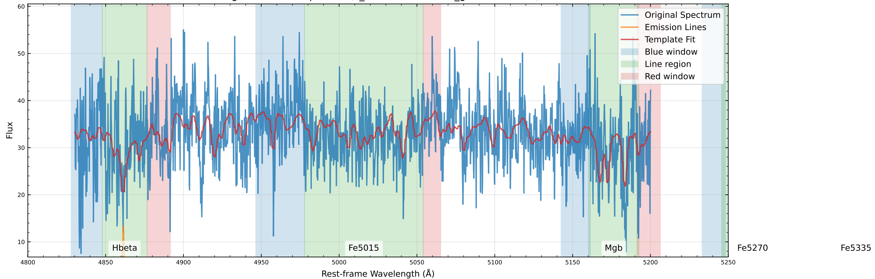
Original Data Comparison (v_star=19.8 km/s, v_gas=97.4 km/s)
