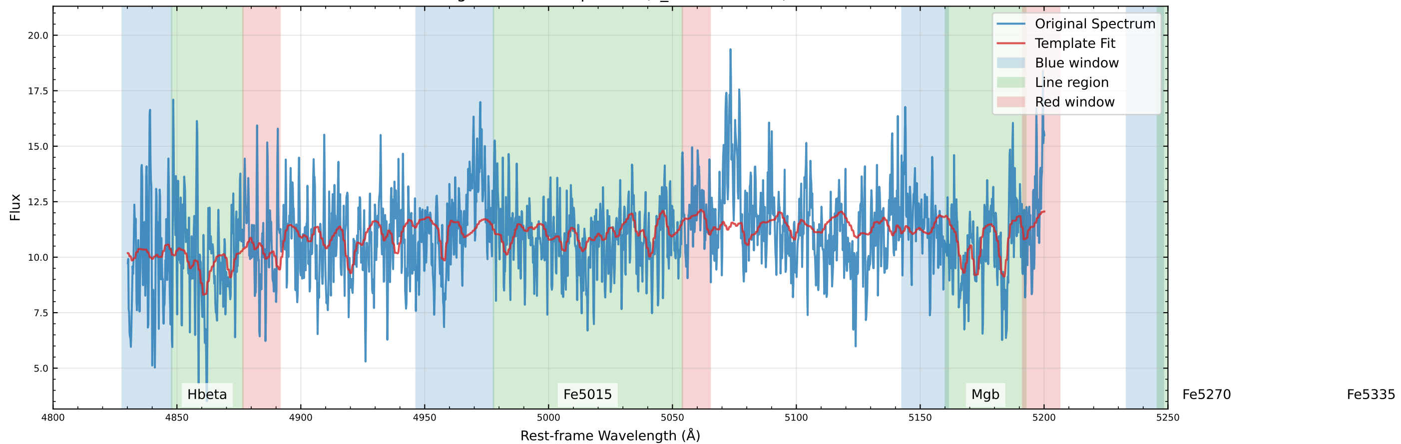
Original Data Comparison (v_star=5.7 km/s)
