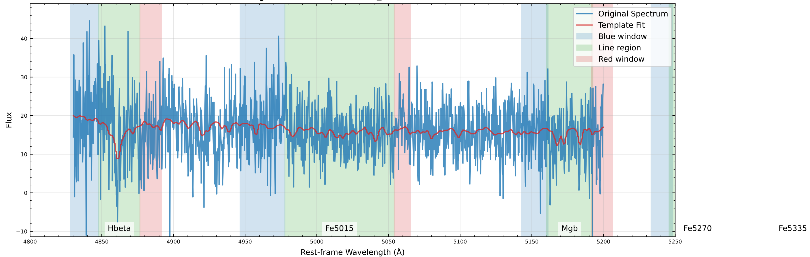
Original Data Comparison (v_star=-41.7 km/s)
