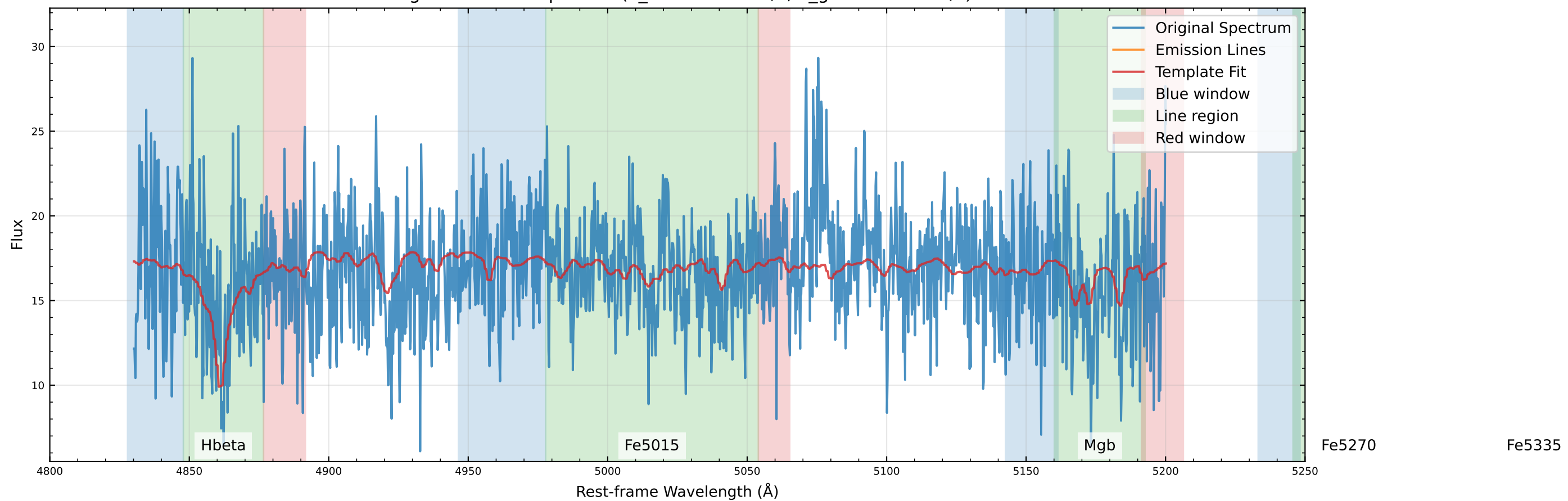
Original Data Comparison (v_star=57.2 km/s, v_gas=109.8 km/s)
