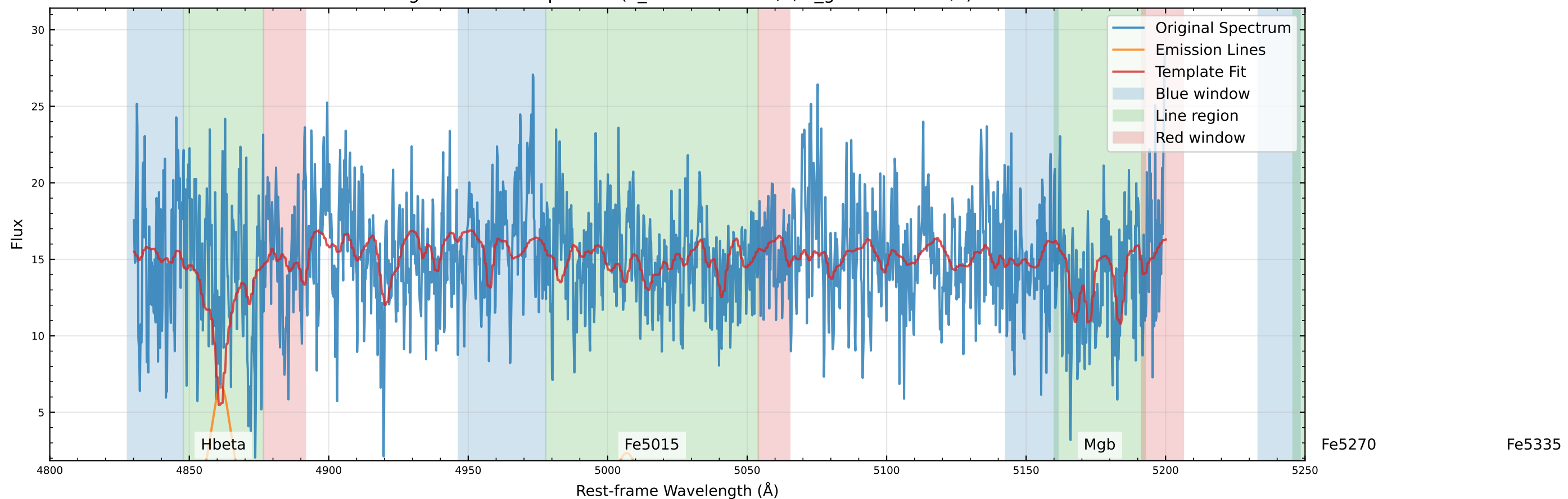
Original Data Comparison (v_star=-73.3 km/s, v_gas=-78.6 km/s)
