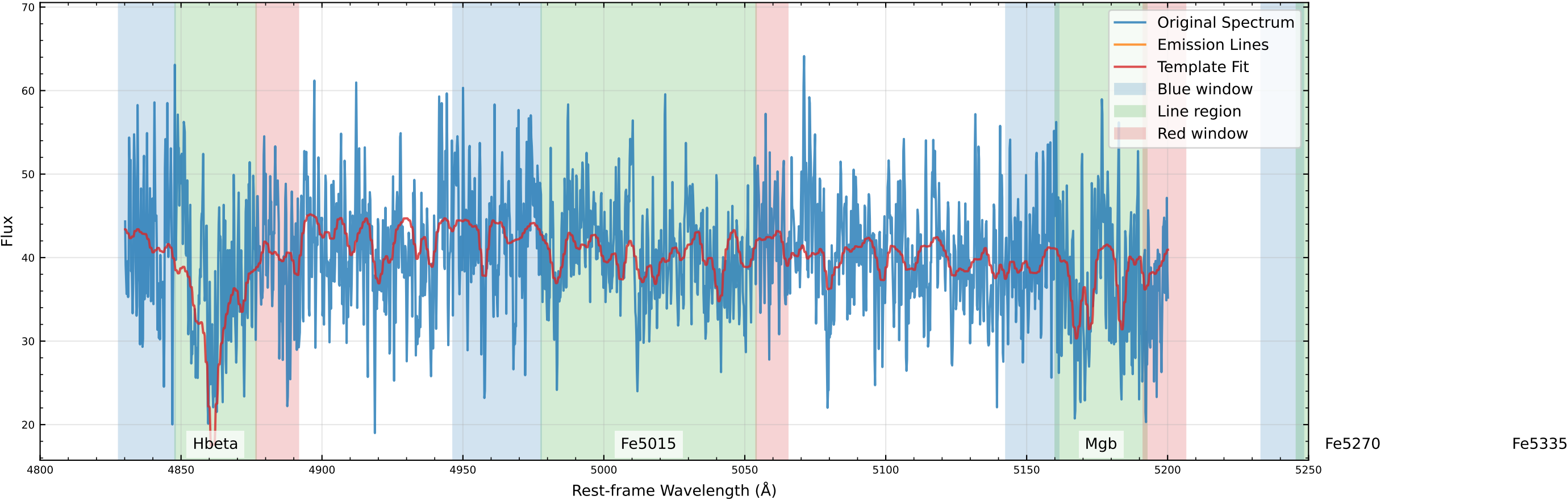
Original Data Comparison (v_star=-20.3 km/s, v_gas=-46.5 km/s)
