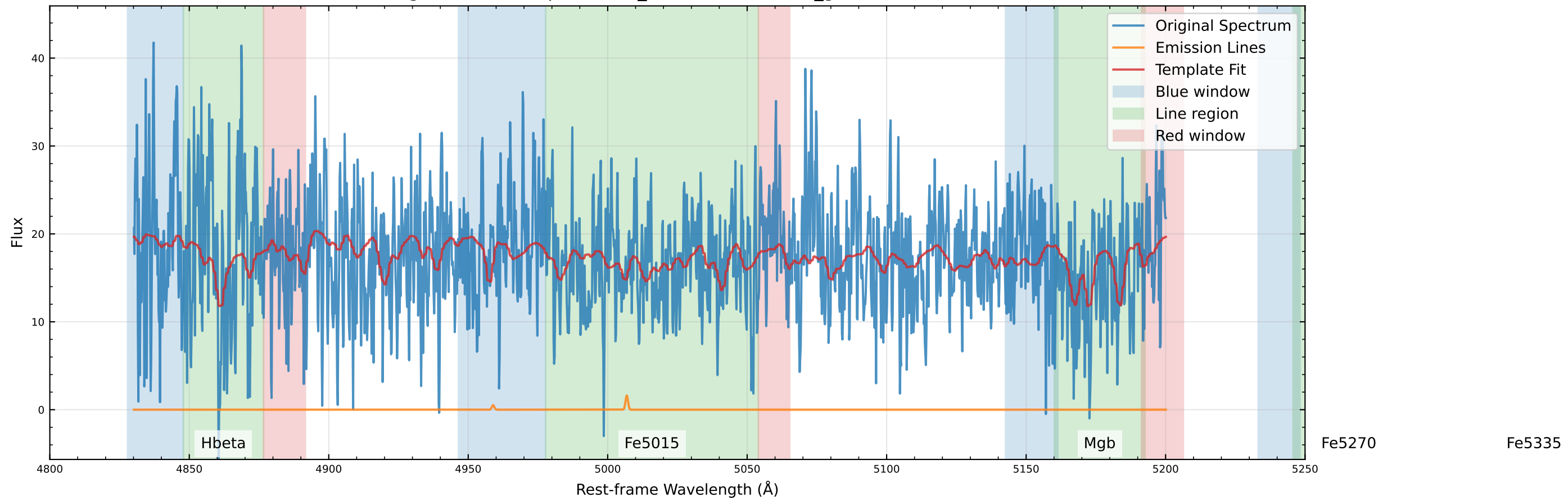
Original Data Comparison (v_star=-32.1 km/s, v_gas=-28.4 km/s)
