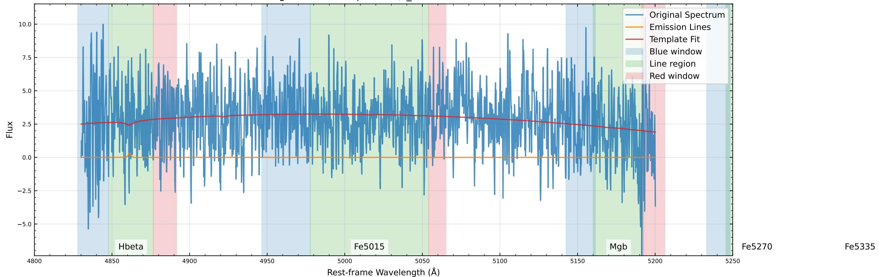
Original Data Comparison (v_star=-119.6 km/s)
