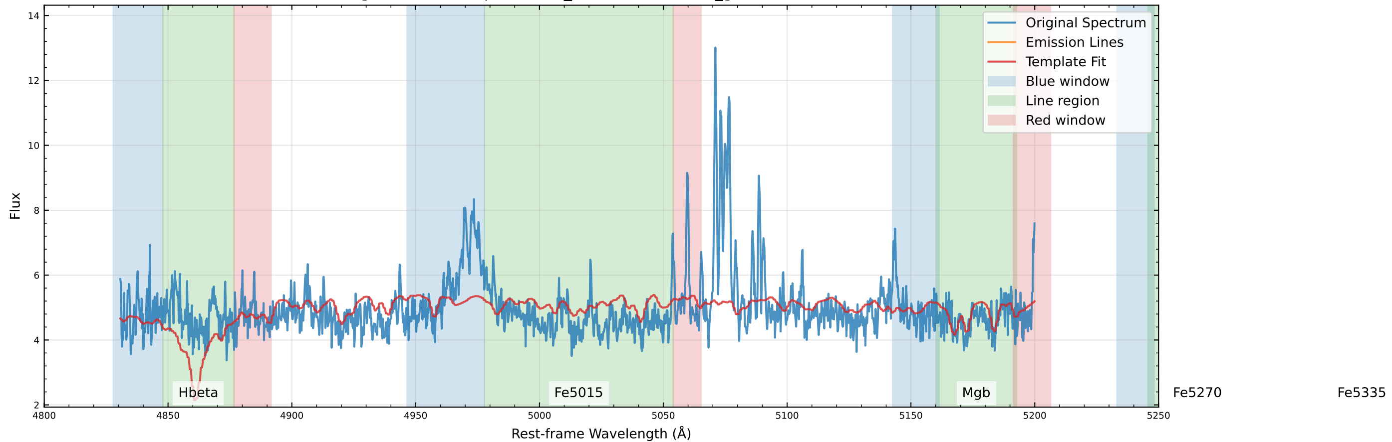
Original Data Comparison (v_star=18.4 km/s, v_gas=-107.3 km/s)
