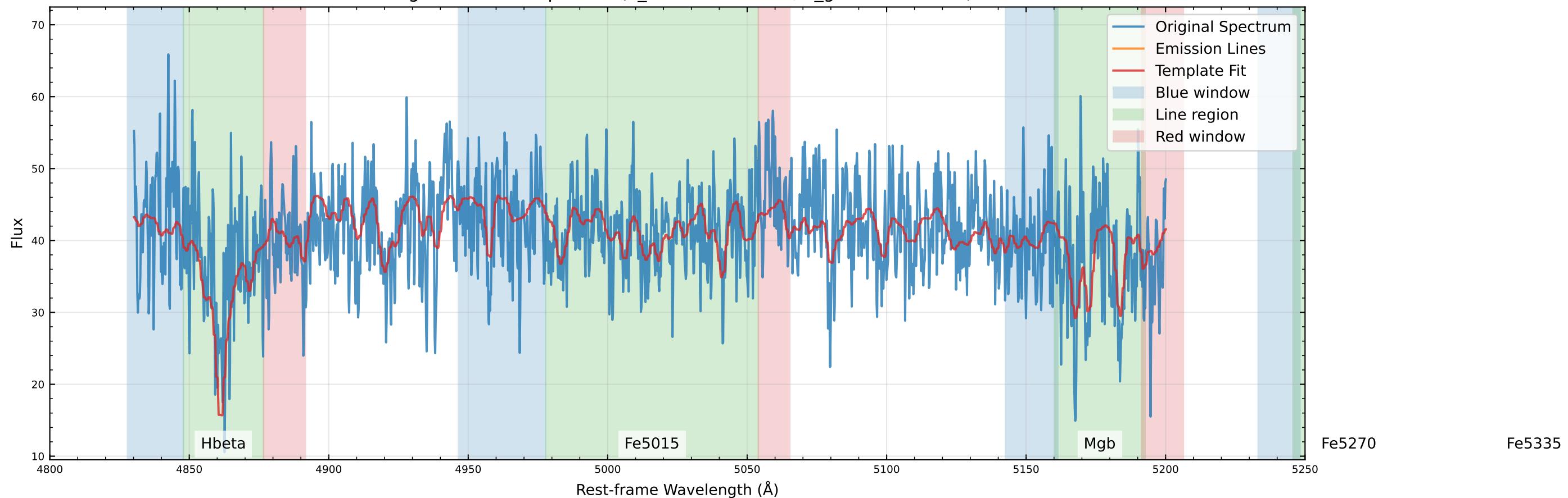
Original Data Comparison (v_star=-15.7 km/s, v_gas=-20.2 km/s)
