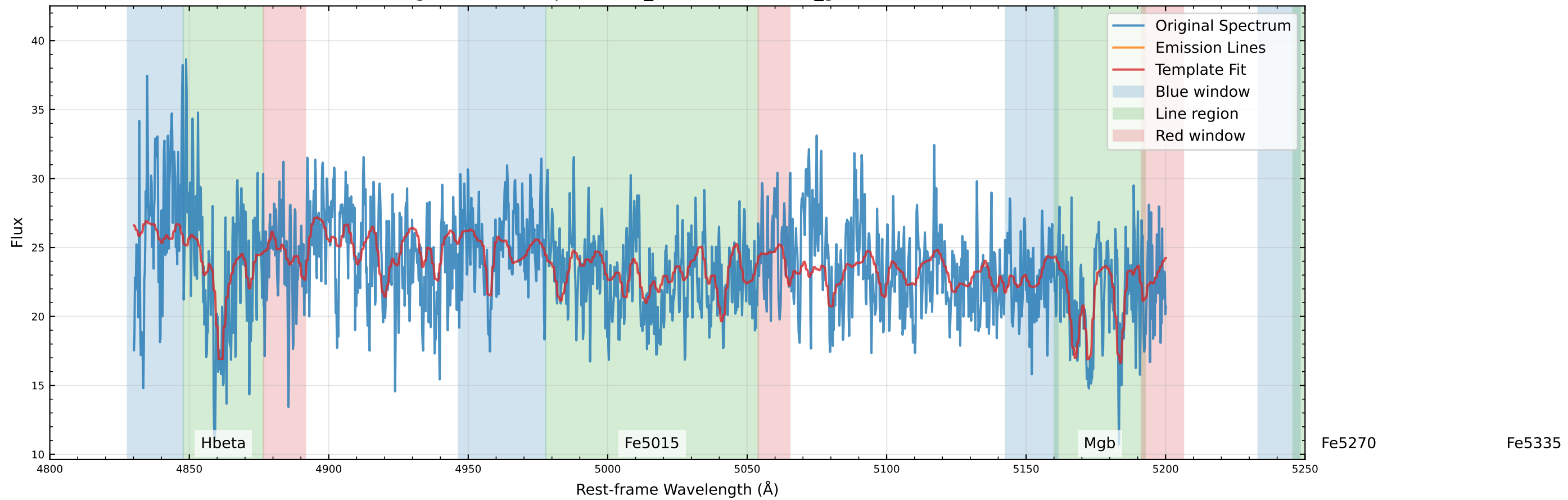
Original Data Comparison (v_star=15.4 km/s, v_gas=31.1 km/s)
