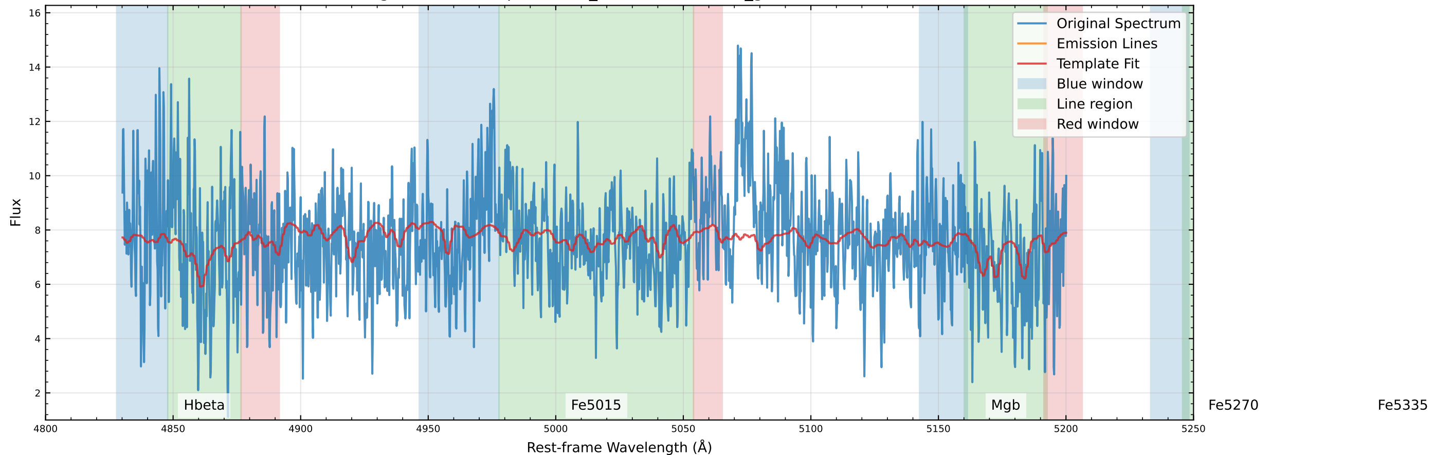
Original Data Comparison (v_star=32.4 km/s, v_gas=38.1 km/s)
