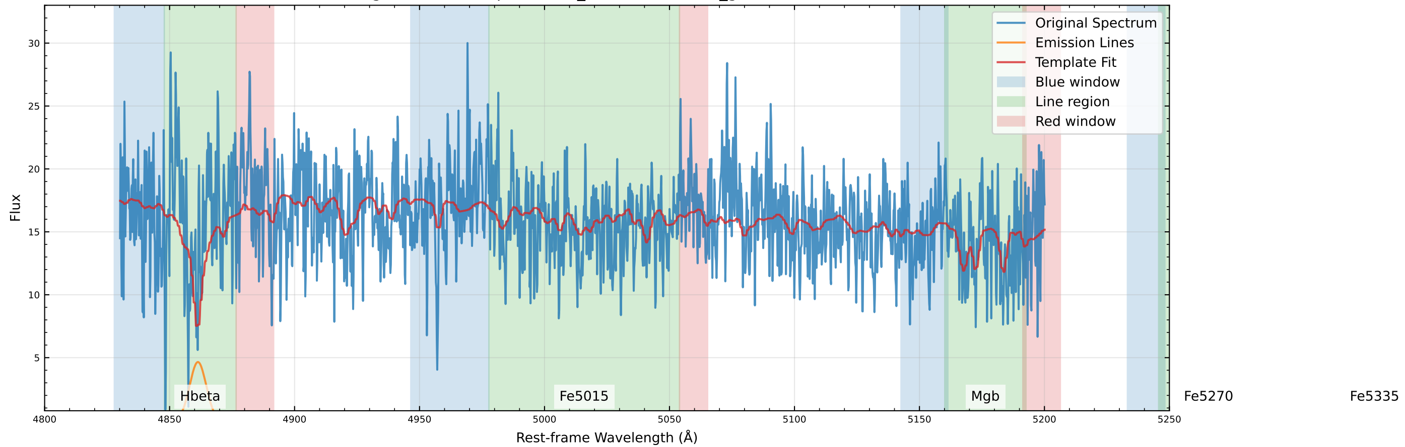
Original Data Comparison ( v_{\text{star}}=0.5 km/s, v_{\text{gas}}=207.1 km/s)
