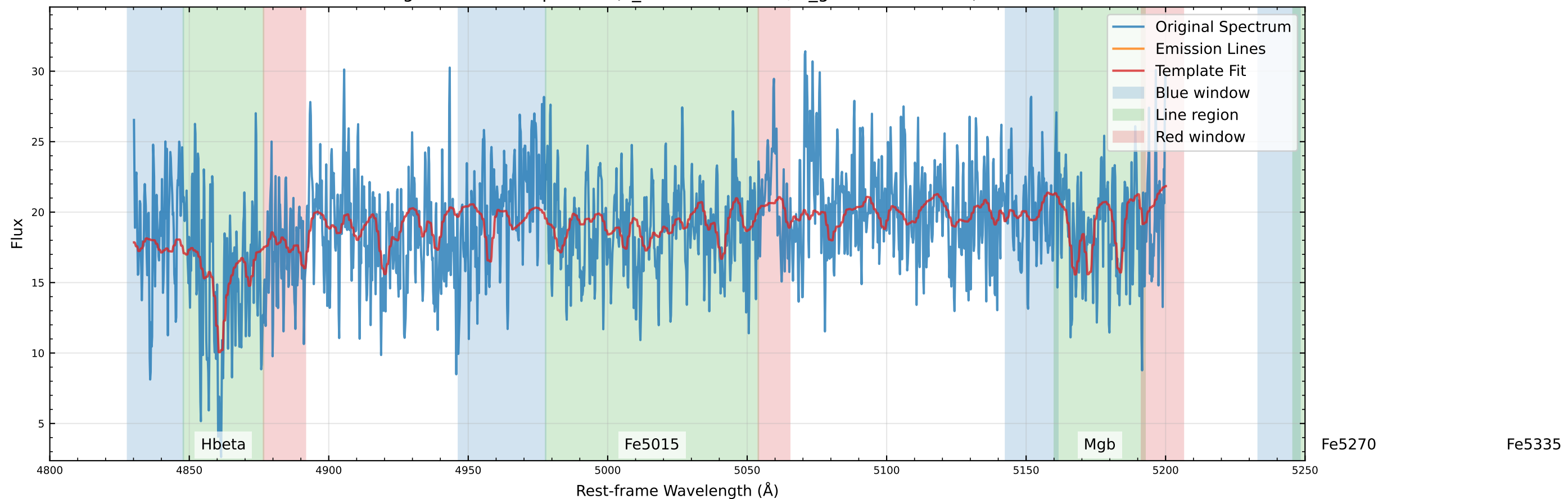
Original Data Comparison (v_star=-17.7 km/s, v_gas=-106.3 km/s)
