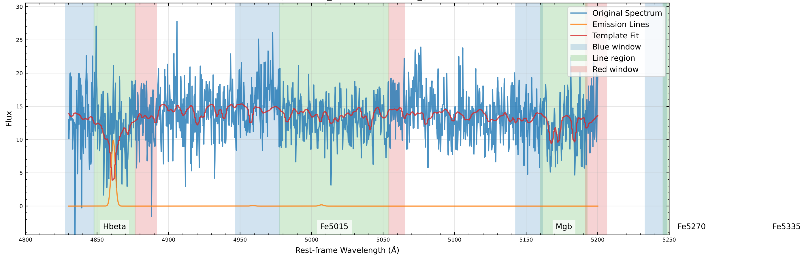
Original Data Comparison (v_star=-29.9 km/s, v_gas=-15.4 km/s)
