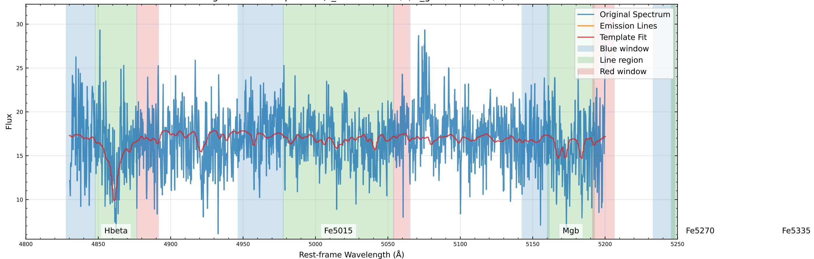
Original Data Comparison ( v_{\text{star}}=57.2 km/s, v_{\text{gas}}=109.8 km/s)
