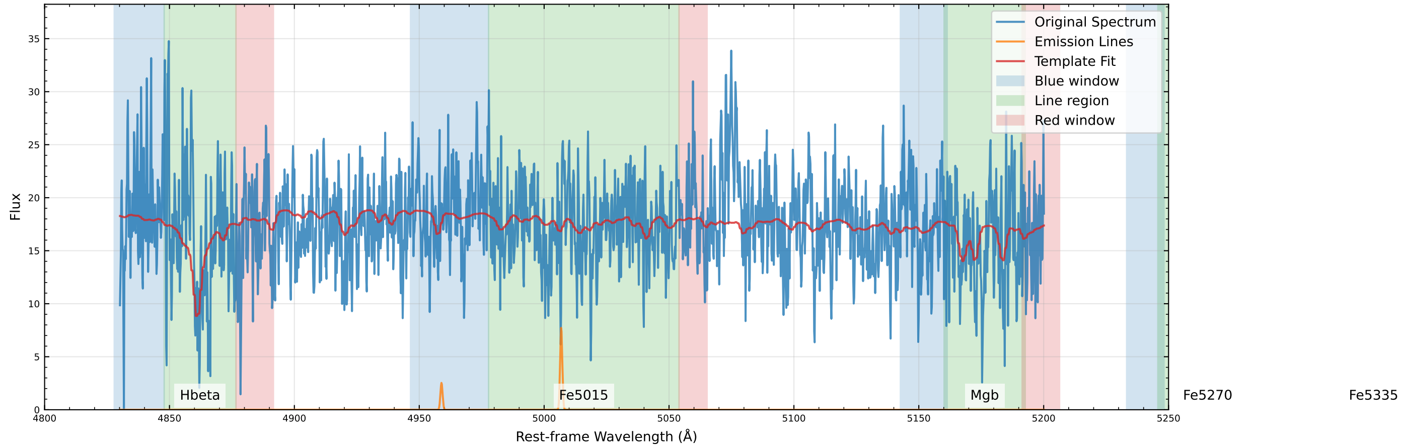
Original Data Comparison (v_star=25.8 km/s, v_gas=52.9 km/s)
