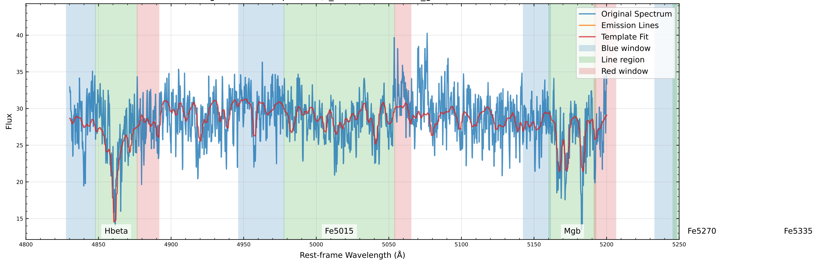
Original Data Comparison (v_star=-17.0 km/s, v_gas=-272.7 km/s)
