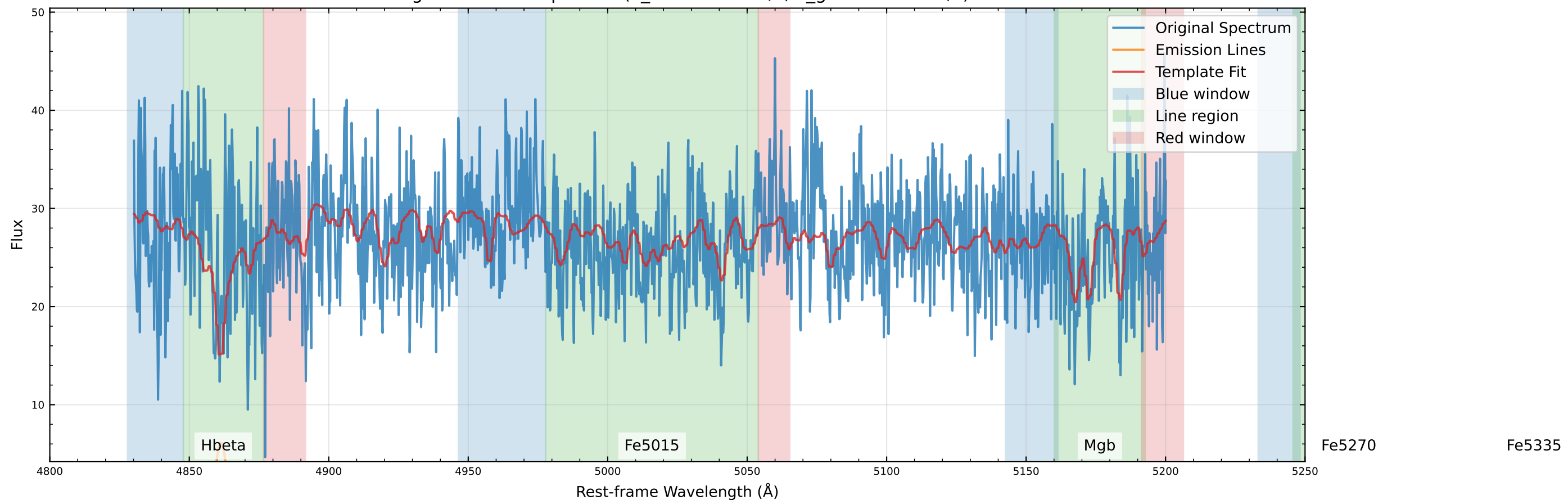
Original Data Comparison (v_star=-2.5 km/s, v_gas=105.8 km/s)
