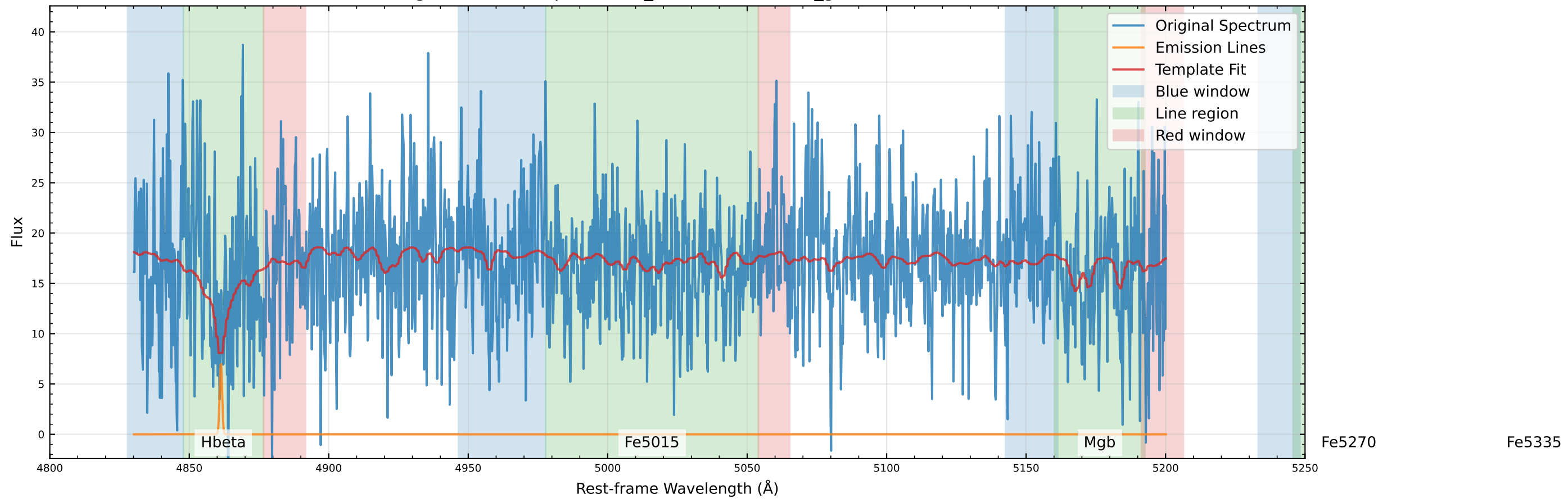
Original Data Comparison (v_star=26.3 km/s, v_gas=90.5 km/s)
