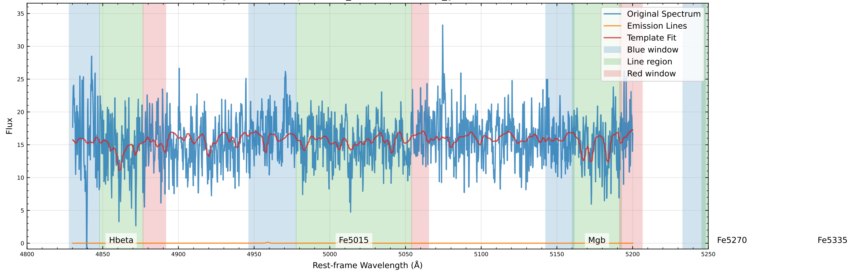
Original Data Comparison (v_star=-27.4 km/s, v_gas=-21.8 km/s)
